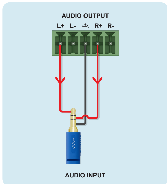
Balanced Phoenix Output to Unbalanced TRS Input
